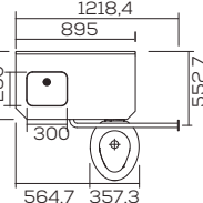
V. SUPERIOR
