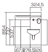
V. FRONTAL
