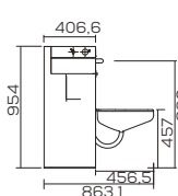
V. LATERAL
