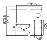
V. LATERAL
