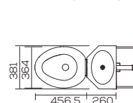
V. SUPERIOR
